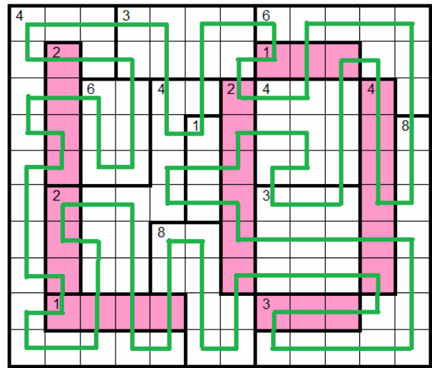
4. Aquapelago (2 body)
