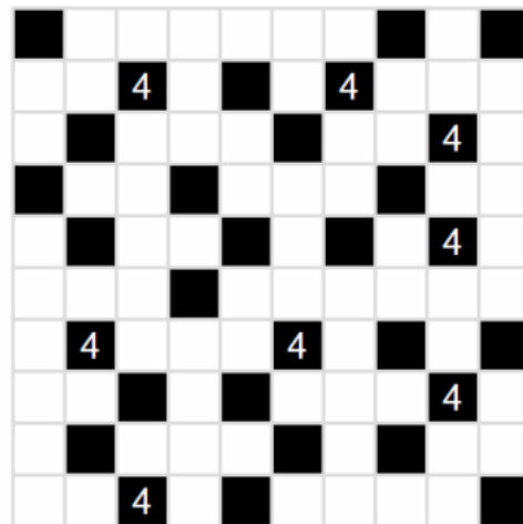
6. Mrakotetris (2 body)
